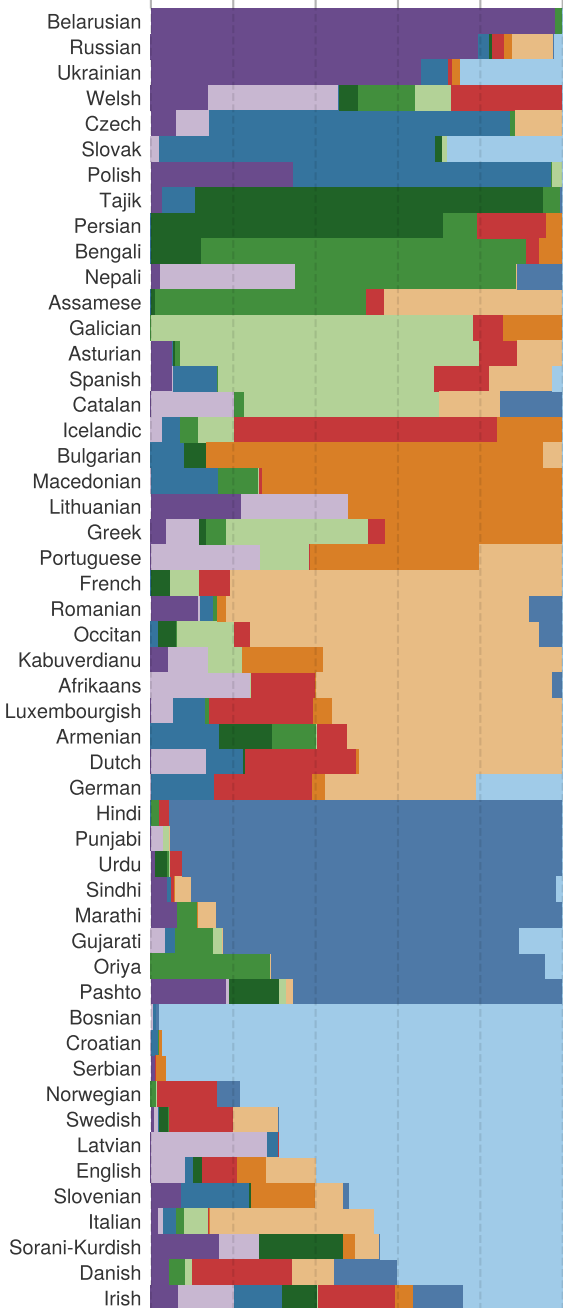
NMF components
