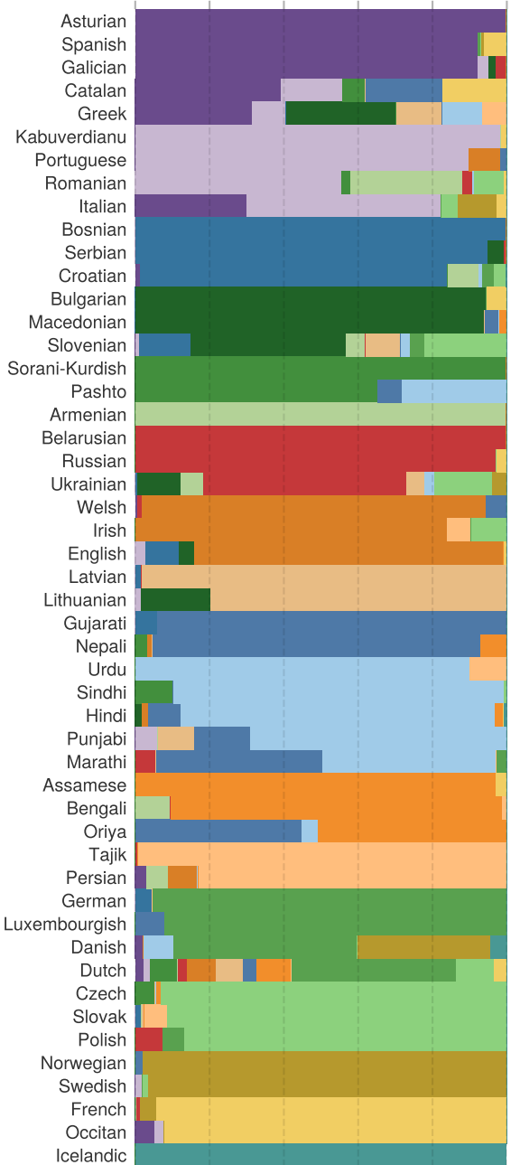
Ancestry proportion
