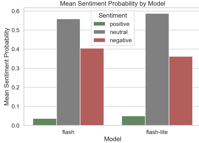
Figure 3: Mean sentiment probabilities by model.
