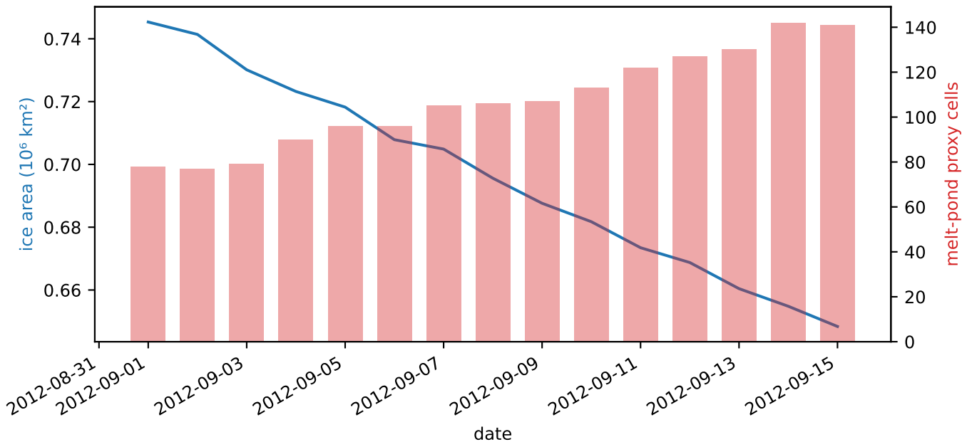
CS3 — sectorial ice area and melt-pond proxy footprint
