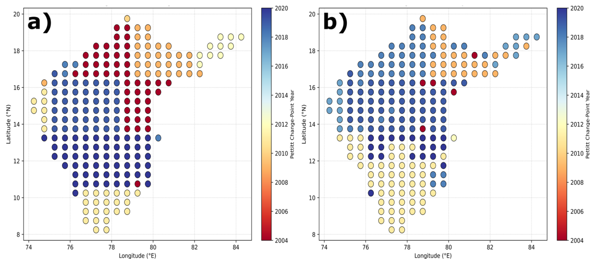
Fig. S4 Spatial distribution of significant breakpoints in post-monsoon groundwater anomaly homogeneity of (a) missing and (b) interpolated data during November as identified using Pettitt's test ( p < 0.05 ).
