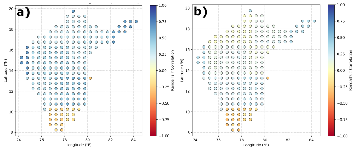
Fig. S1 Spatial distribution of post-monsoon groundwater anomaly trends of (a) missing and (b) interpolated data during October based on Kendall's tau values, indicating the strength and direction of groundwater change.
