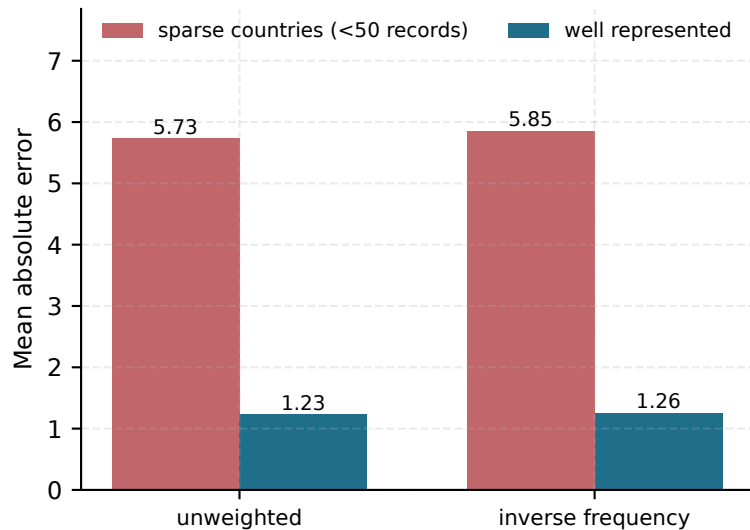
Error by representation, and the effect of weighting
