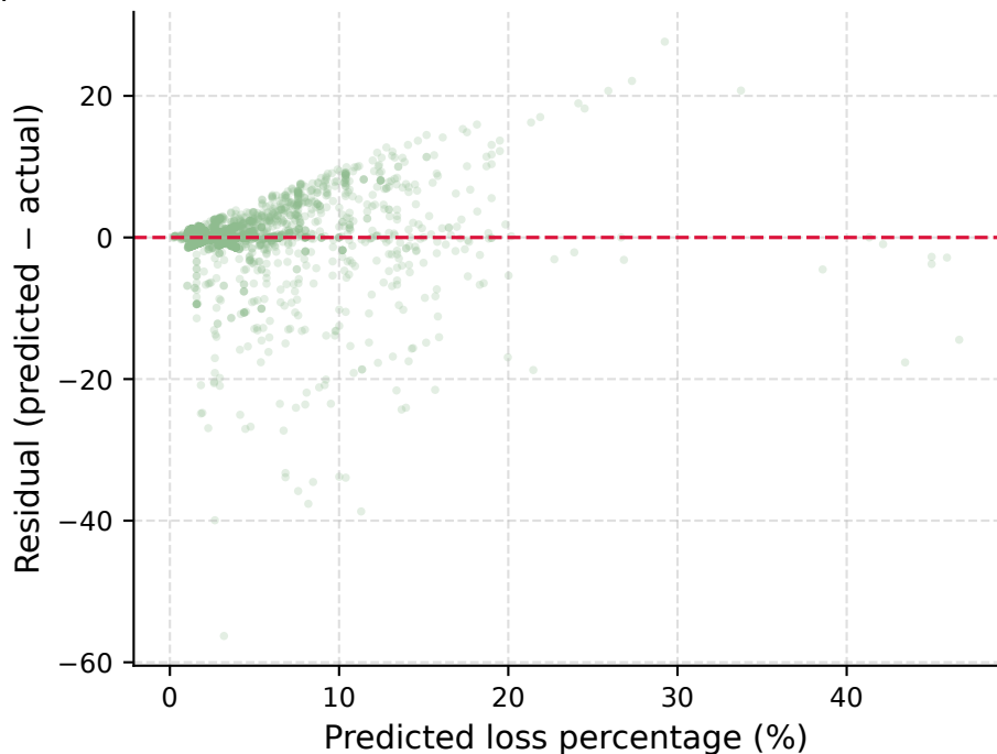
Residuals vs Predicted — Random Forest pooled over all held-out records: mean residual = +0.077, sd = 3.838
