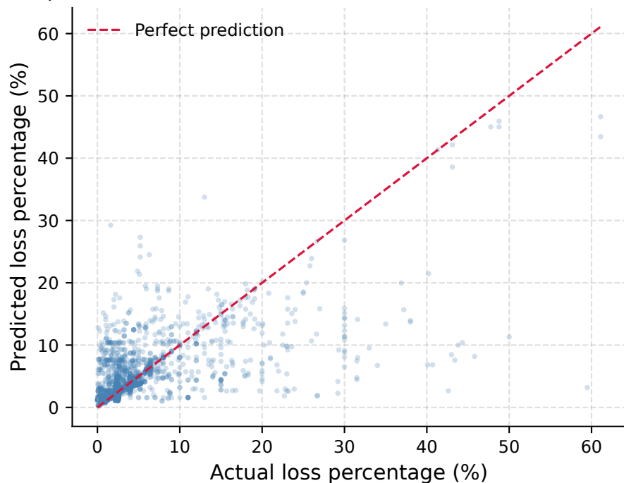
Predicted vs Actual — Random Forest pooled over all held-out records: R^2 = 0.378 , MAE = 1.549
