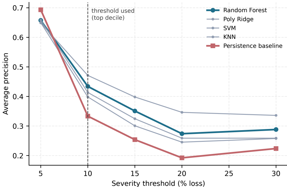
F9. Average precision across severity thresholds. Below about 8% the baseline is ahead; the models' advantage is specific to severe losses.
