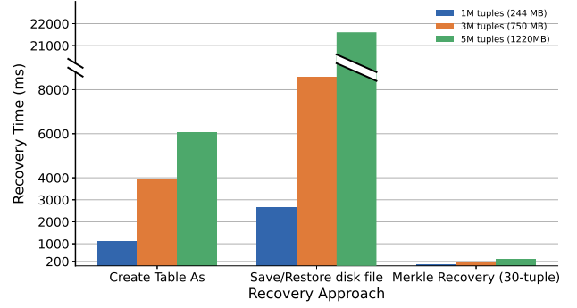
Figure 13: Performance comparison of Corruption Recovery approaches
