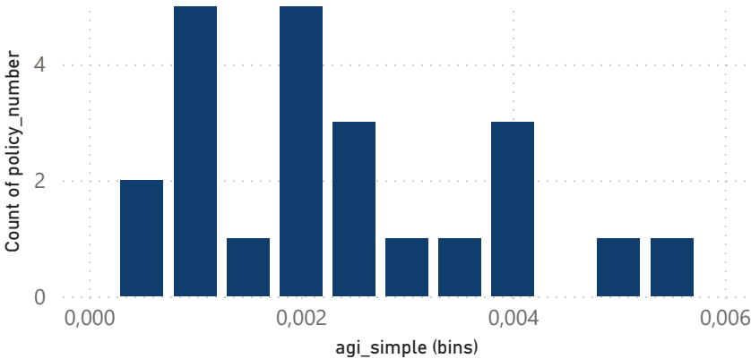
Count of policy_number by agi_simple (bins)
