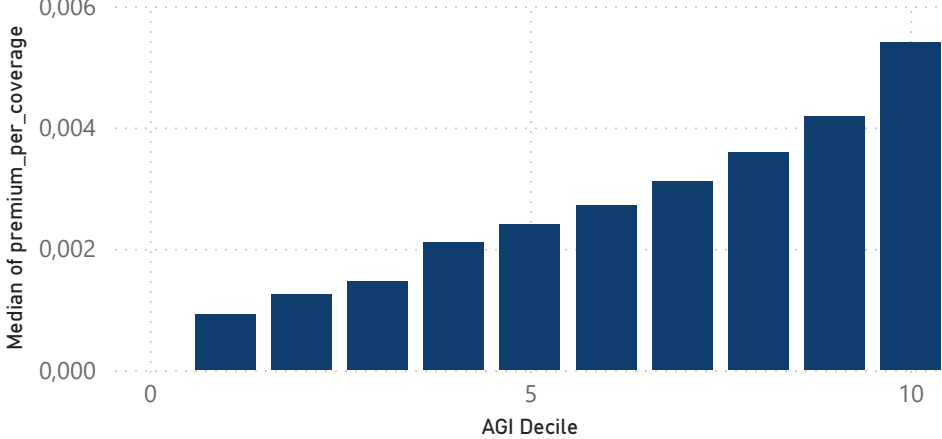
Median of premium_per_coverage by AGI Decile
