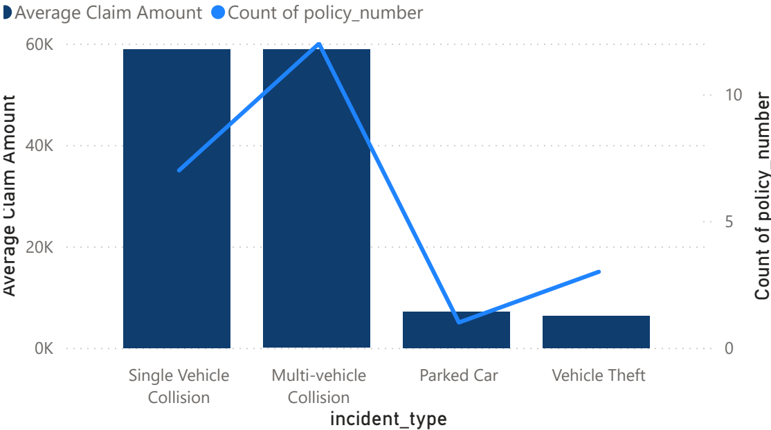
Average Claim Amount and Count of policy_number by incident_type
