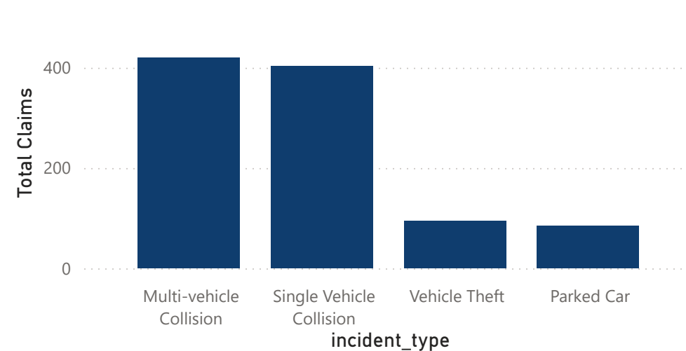
Total Claims by incident_type
