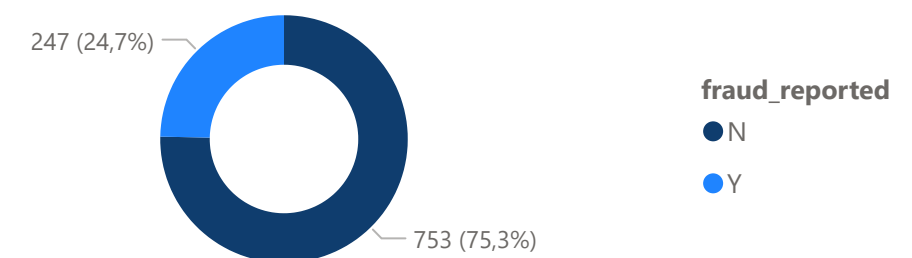
Total Claims by fraud_reported
