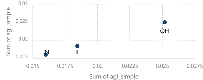
Sum of agi_simple and Sum of agi_simple by policy_state
