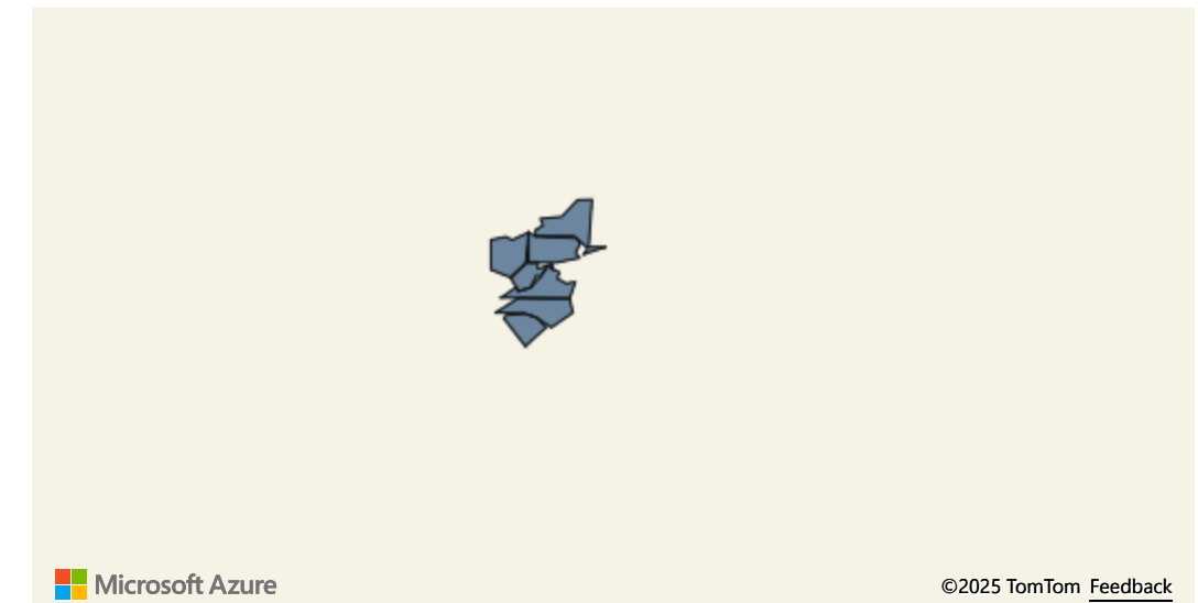
Total Claims by fraud_reported
