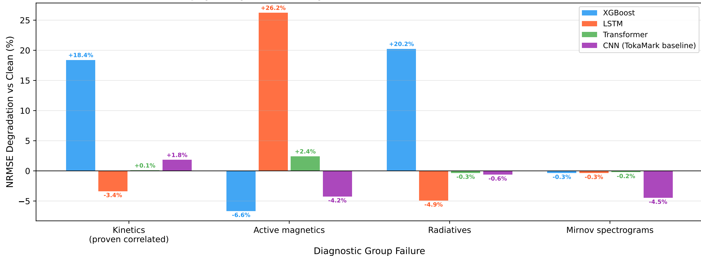
Correlated Diagnostic Group Failure (physically motivated by observed NaN correlation in MAST data)
