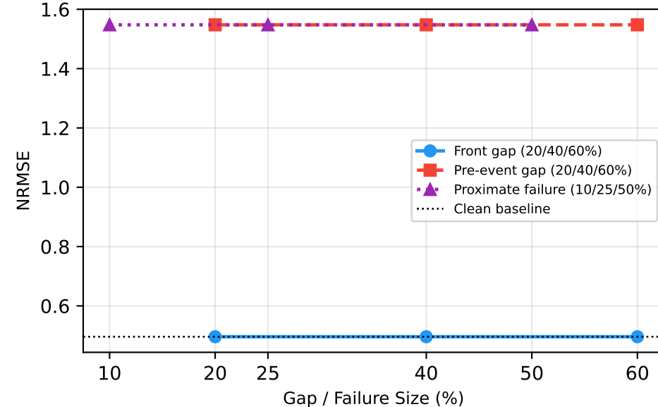
LSTM
