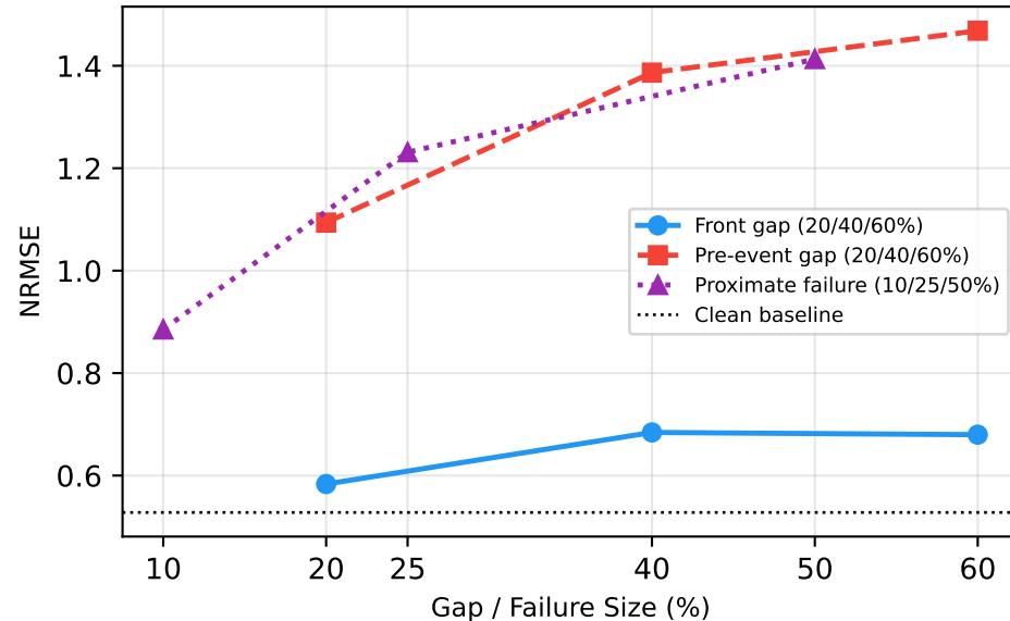
CNN (TokaMark baseline)
