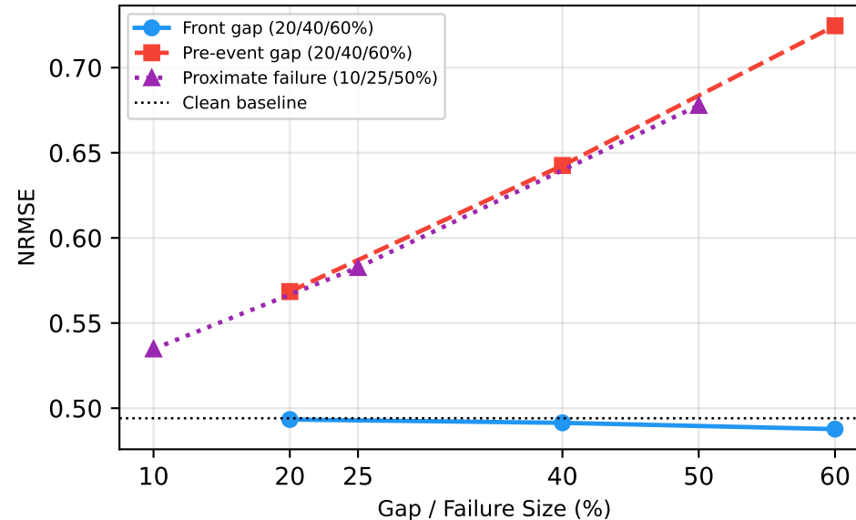
XGBoost
