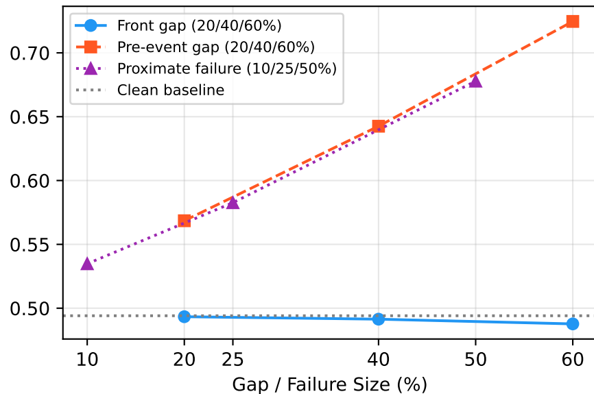
XGBoost
