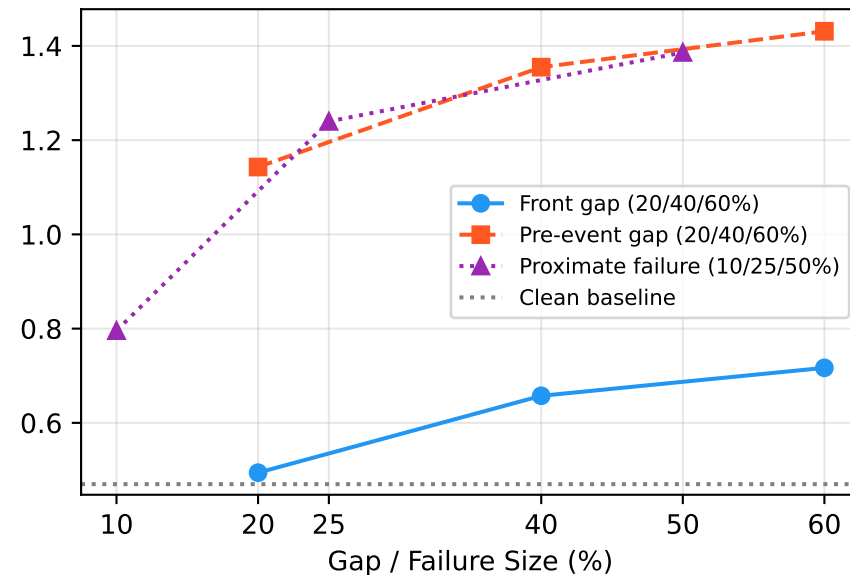
Transformer
