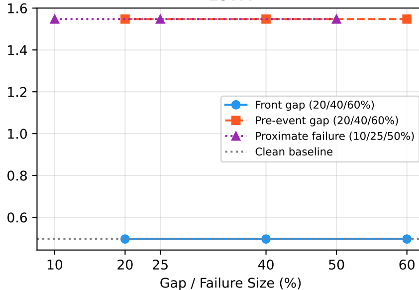
LSTM
