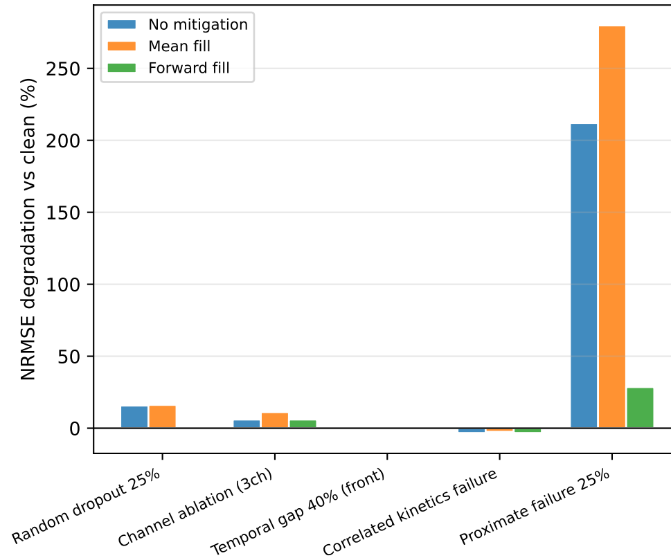
LSTM
