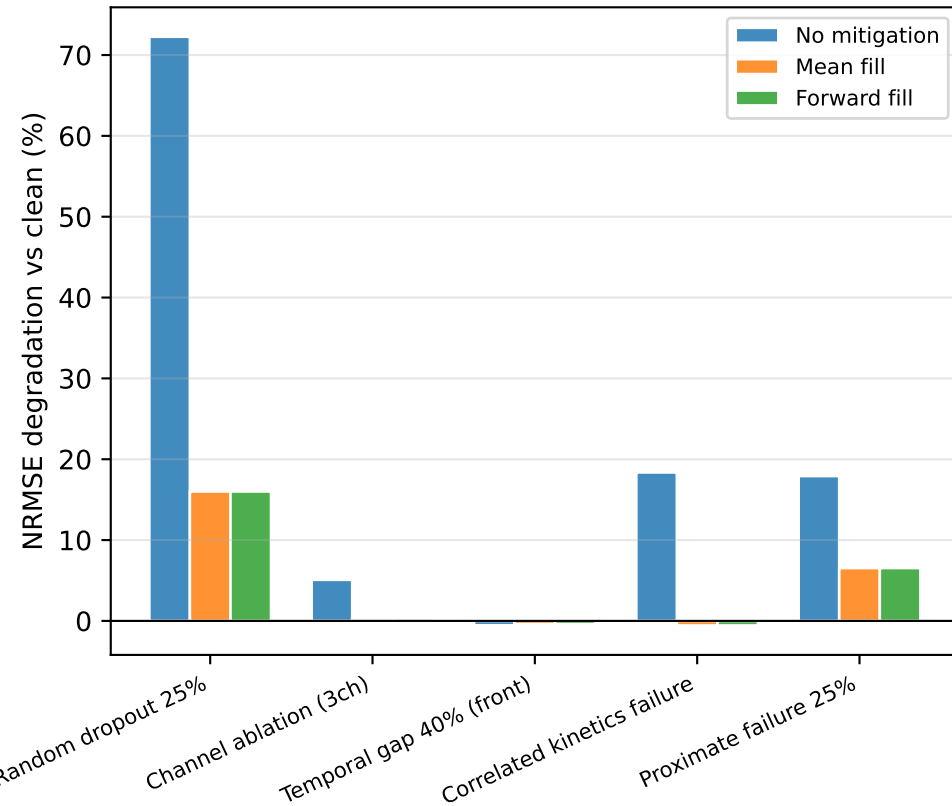
XGBoost
