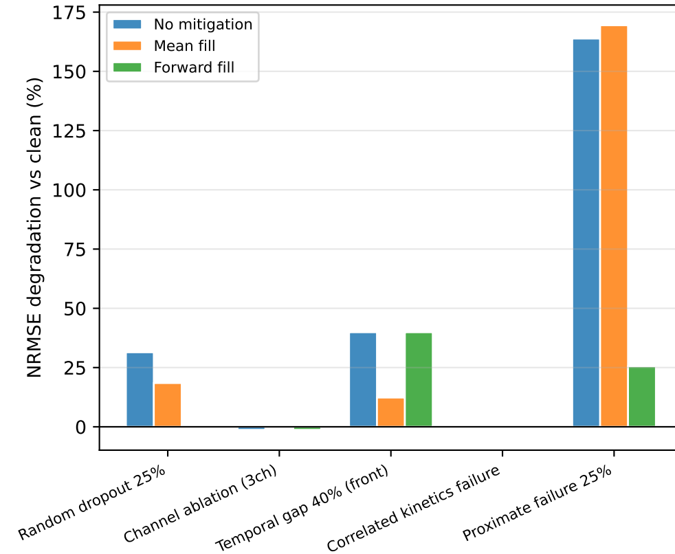
Transformer
