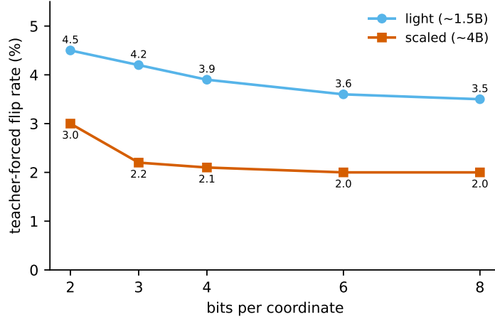
Figure 4: The bit-rate dose-response is monotone but buffered. Teacher-forced arg-max flip rate versus channel bit-rate on MBPP+. Flips increase monotonically as bits fall, on both tiers, and scaled stays below light at every rate; yet even 2-bit quantization adds only \sim 1 pp—the REF margin distribution buffers the flip rate against the growing perturbation.
