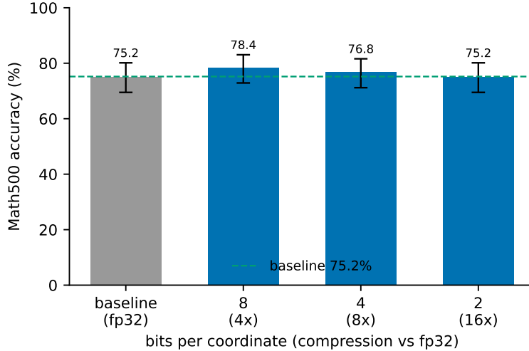
Figure 5: Independent historical corroboration: T4 fp32 Math500 sampled accuracy versus bit rate ( n = 250 , Wilson 95% intervals). The ladder is non-monotonic and every interval overlaps the baseline; these unpaired sampled runs support “no detected degradation,” not equivalence.
