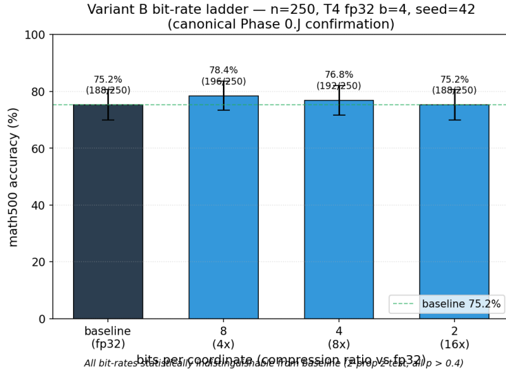
Figure 1: Math500 accuracy versus TurboQuant-MSE bit-rate at n=250 under sampled decoding. The curve is flat from the unquantized baseline through 16\times compression; every bit-rate lies within sampling noise of the baseline. Under greedy decoding a stricter paired equivalence test is inconclusive (Section 4.3).
