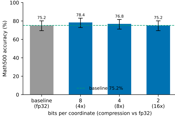
Figure 3: Independent historical corroboration: T4 fp32 Math500 sampled accuracy versus bit rate ( n = 250 , Wilson 95% intervals). The ladder is non-monotonic and every interval overlaps the baseline; these unpaired sampled runs support “no detected degradation,” not equivalence.
