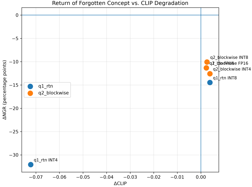
Figure 4: Scatter plot of \Delta\text{NGR} vs. \Delta\text{CLIP} illustrating structural degradation versus concept retention.
