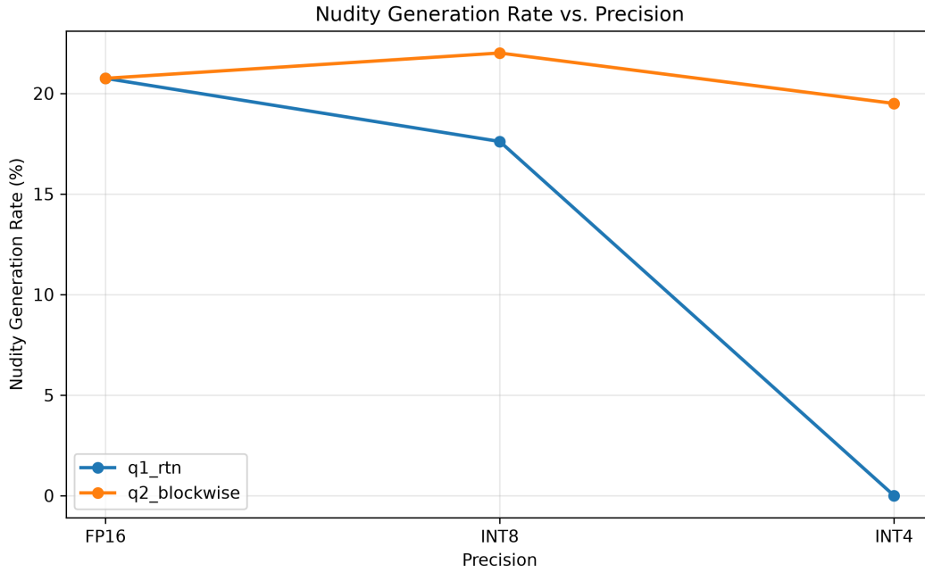
Figure 1: Nudity Generation Rate vs. Precision for q1_rtn and q2_blockwise methods.
