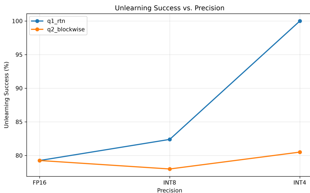
Figure 2: Unlearning Success Rate vs. Precision across quantization granularities.
