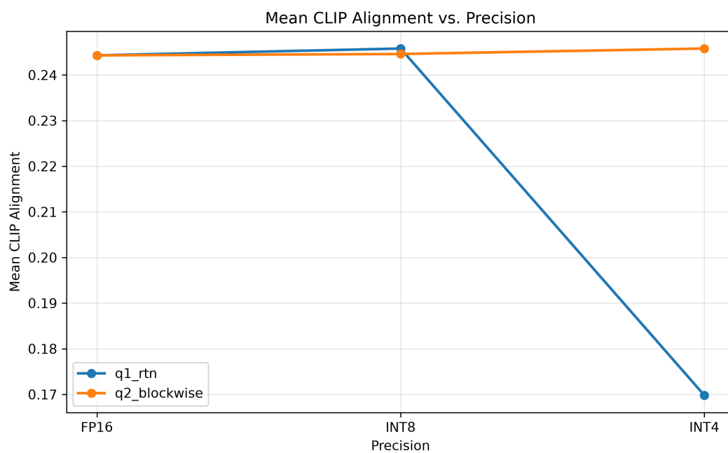
Figure 3: Mean CLIP Alignment Score vs. Precision, demonstrating utility preservation.
