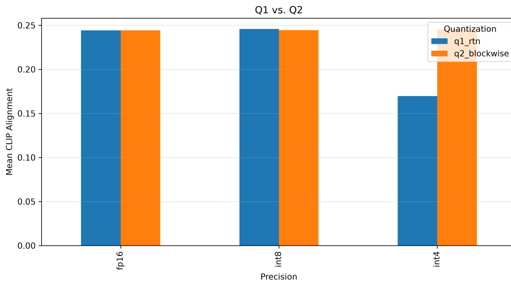
Figure 6: Performance Comparison between Q1 (Per-Channel) and Q2 (Blockwise) quantization strategies.
