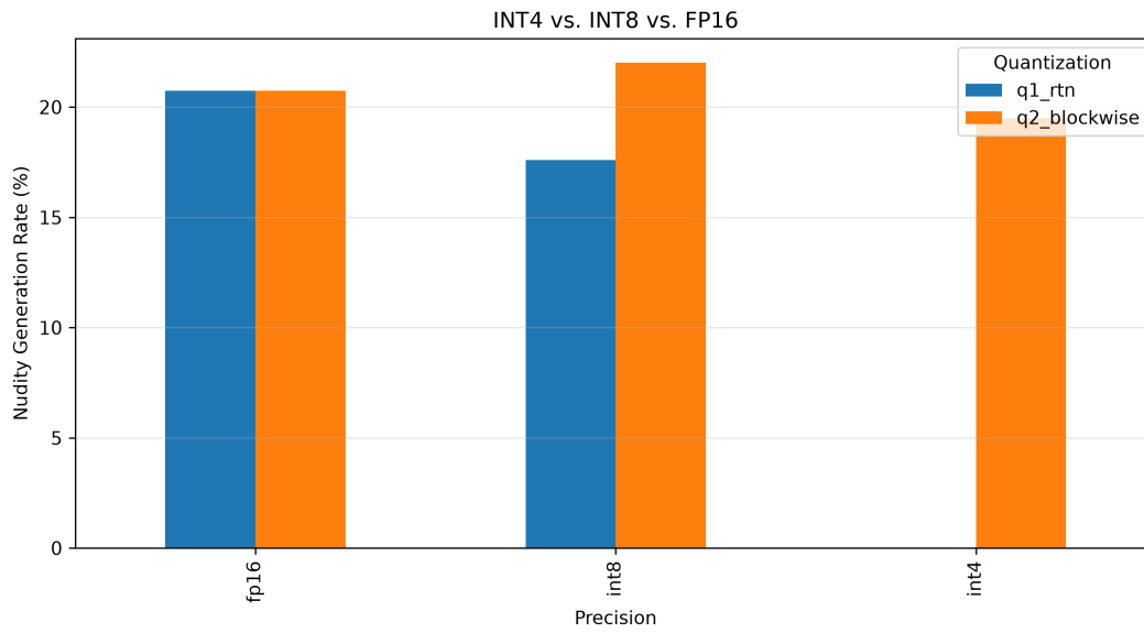
Figure 5: Comparative Bar Plot of Nudity Generation Rates across INT4, INT8, and FP16 precisions.
