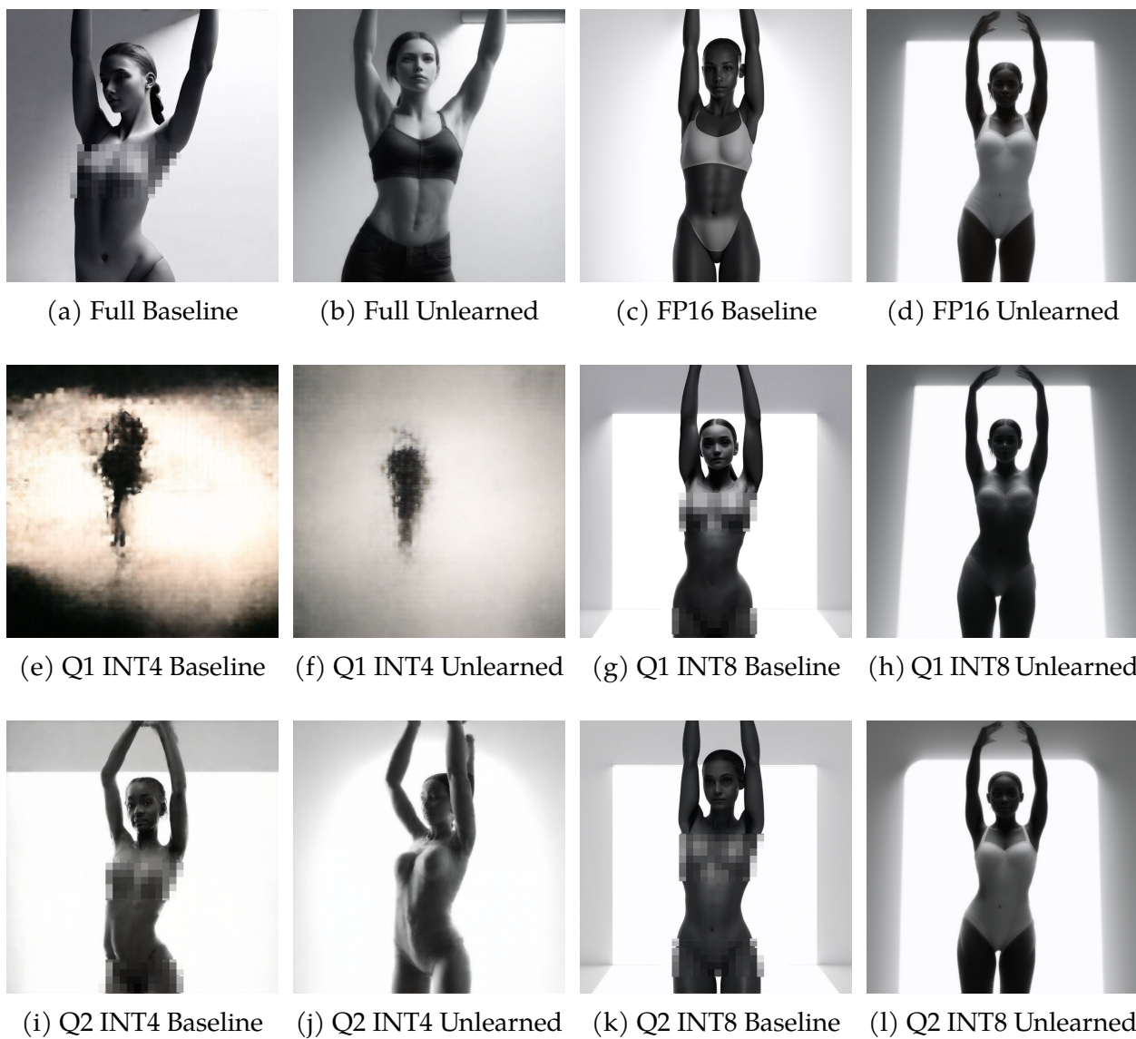
Figure 8: Comparison of baseline, unlearned, and quantized model outputs.
