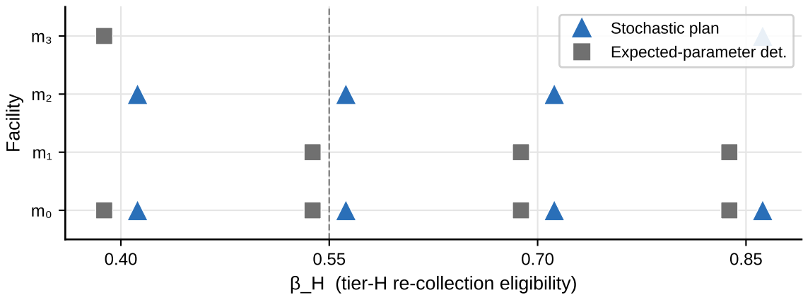
(c) Facility selection by plan vs \beta_H
