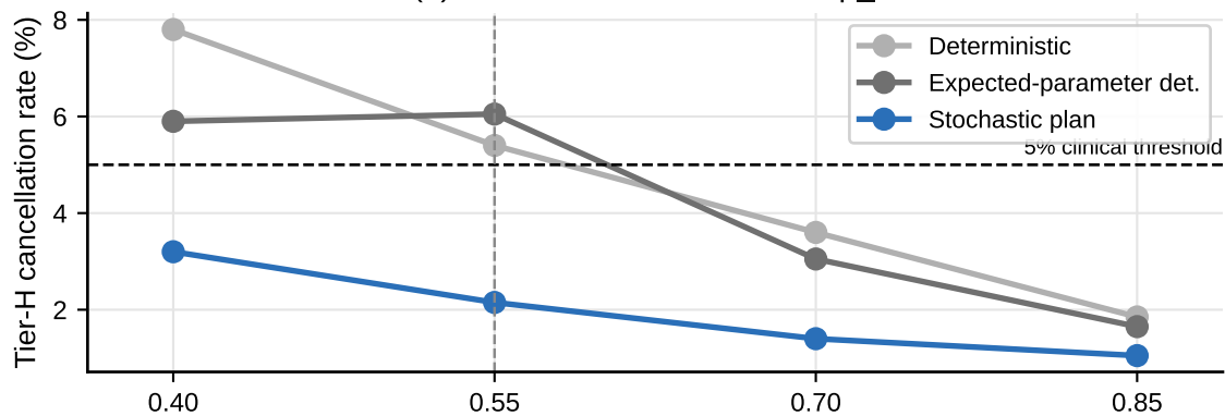
(b) Tier-H cancellation rate vs \beta_H
