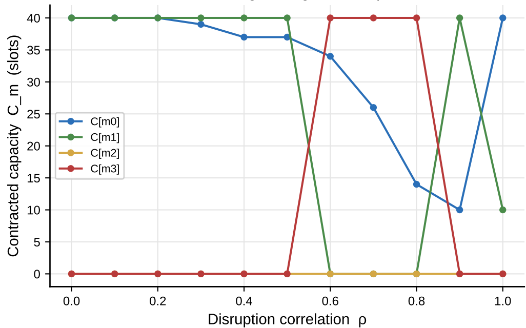
First-stage design across \rho
