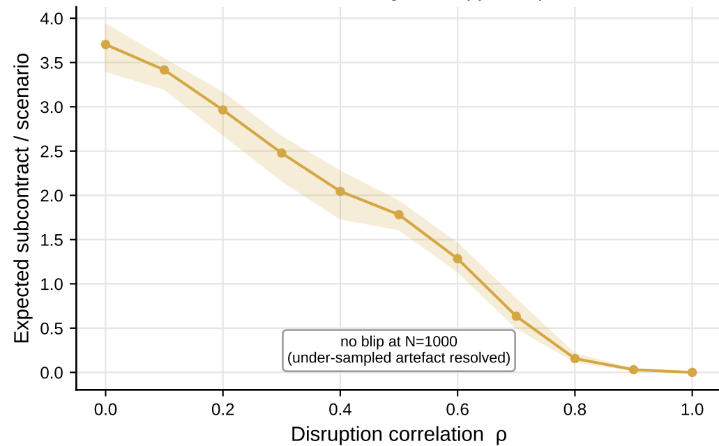
Subcontracting trace ( q=0.15 )
