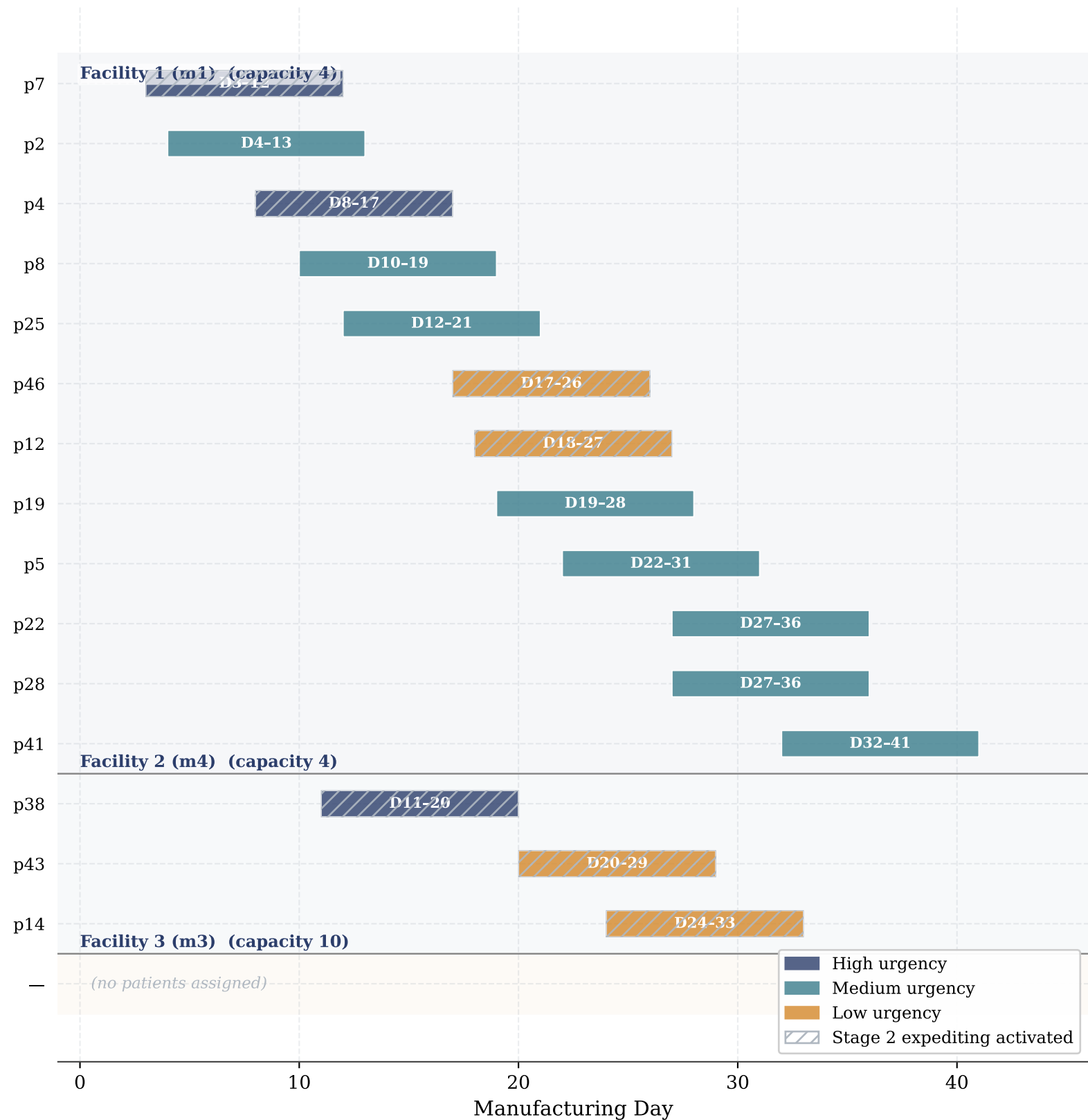
Manufacturing Schedule — Gantt Chart ( N = 15 , two-stage stochastic, seed=42; overlapping bars = concurrent slots)
