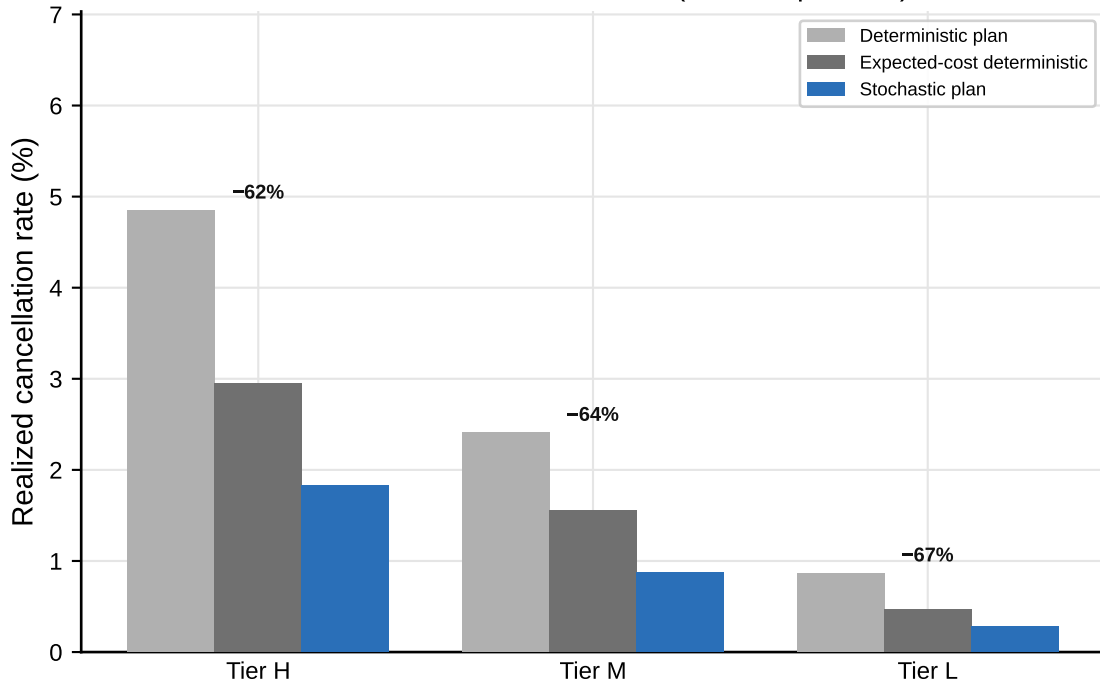
Tier-stratified cancellation rate (N = 200 patients)
