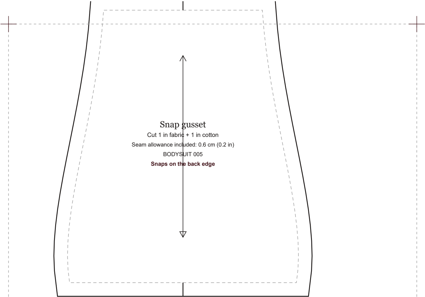
BODYSUIT 005 · Bodysuit · V-Neck · Closed Back · scale 1:1 · 104.6 × 88.1 cm (41.2 × 34.7 in)
