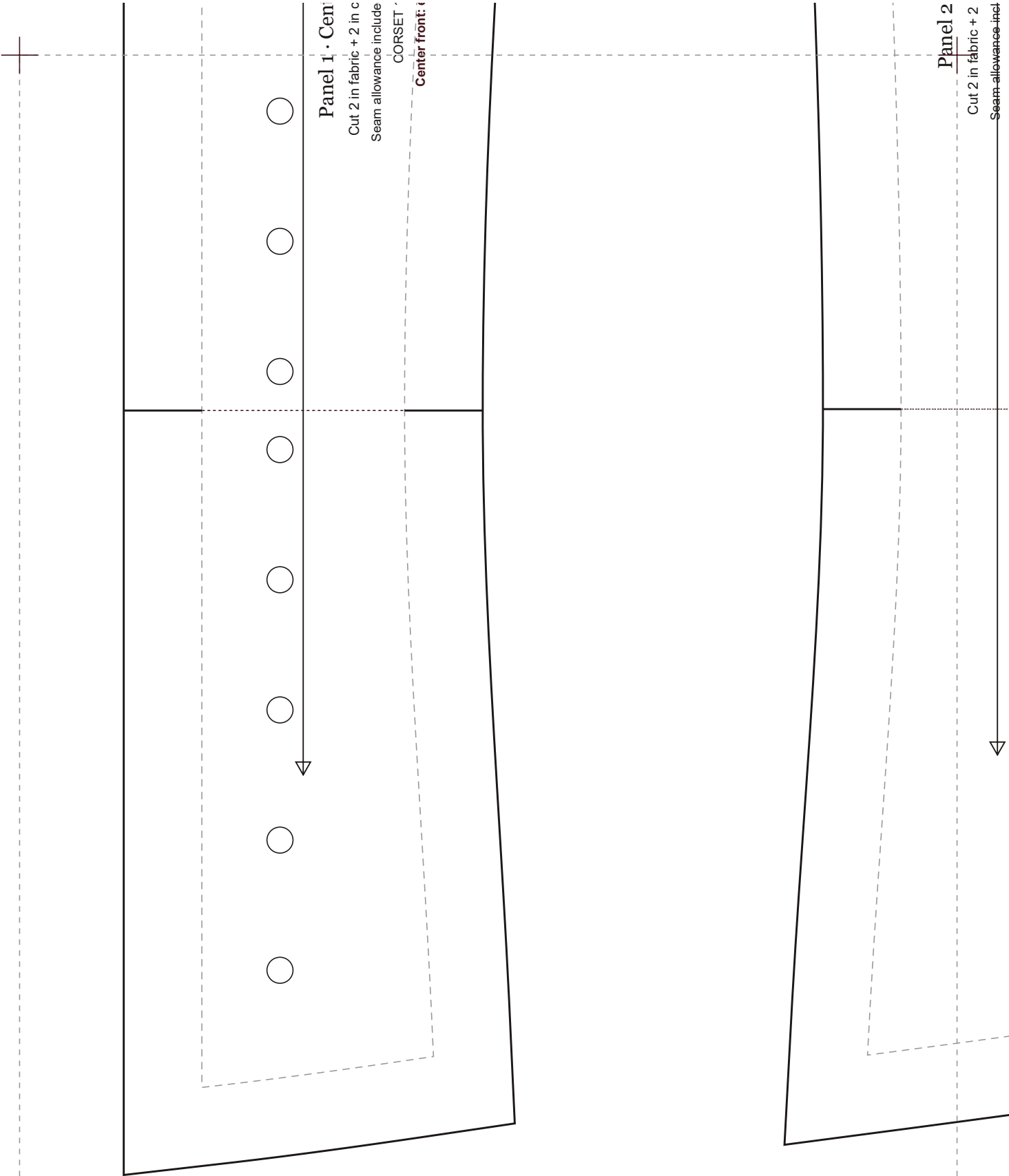
CORSET 110 · Overbust with Front and Back Lacing · 8 Panels · scale 1:1 · 96.4 × 48.2 cm (37.9 × 19.0 in)
