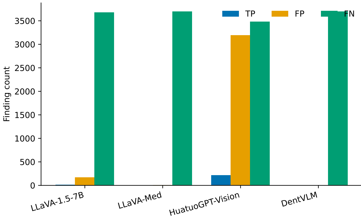
Confusion components (TP / FP / FN) — DENTEX / cot TN omitted: it dwarfs these on the negative-heavy slot grid
