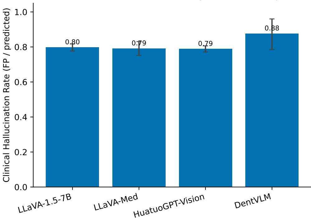
Clinical Hallucination Rate by model — Tufts / zero_shot (lower is better; bars with error = image-level bootstrap 95% CI)
