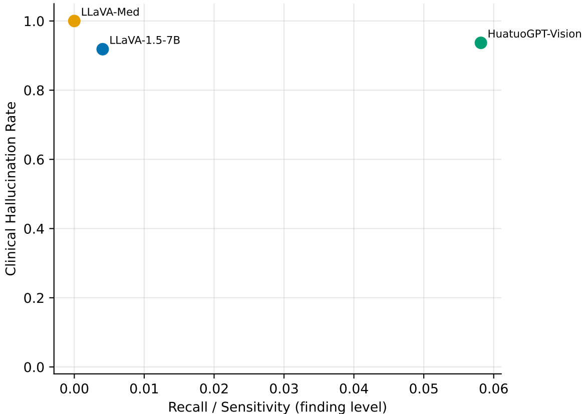
Hallucination vs recall — DENTEX / cot ideal = high recall (right), low CHR (bottom)
