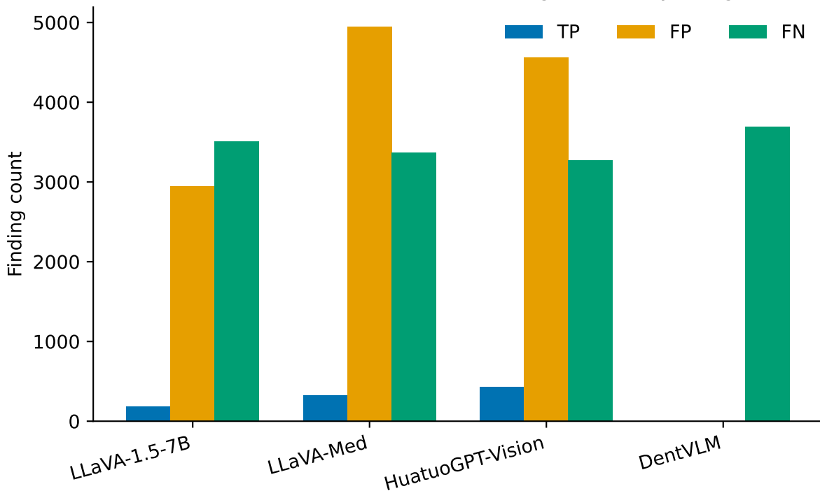
Confusion components (TP / FP / FN) — DENTEX / few_shot TN omitted: it dwarfs these on the negative-heavy slot grid
