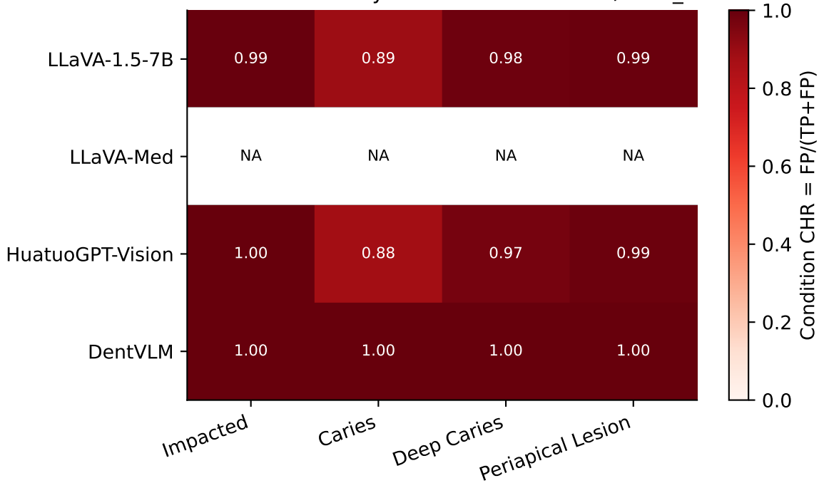
Hallucination RATE by condition — DENTEX / zero_shot
