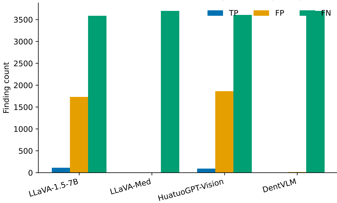
Confusion components (TP / FP / FN) — DENTEX / zero_shot TN omitted: it dwarfs these on the negative-heavy slot grid
