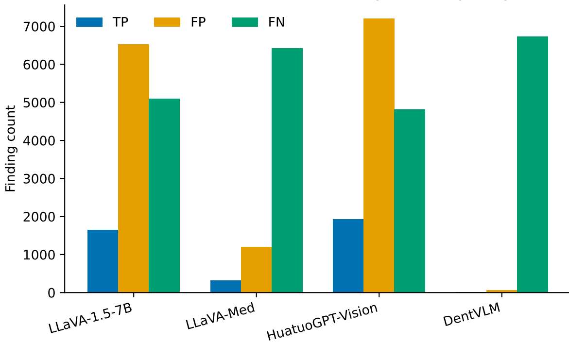
Confusion components (TP / FP / FN) — Tufts / zero_shot TN omitted: it dwarfs these on the negative-heavy slot grid
