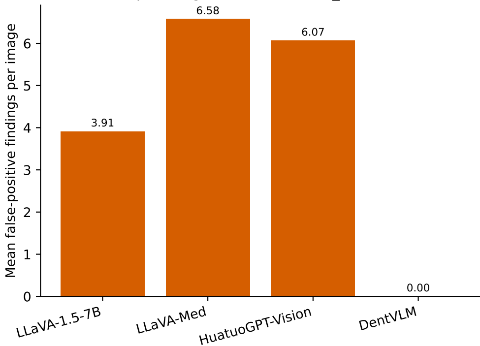
Hallucinations per image — DENTEX / few_shot (lower is better)
