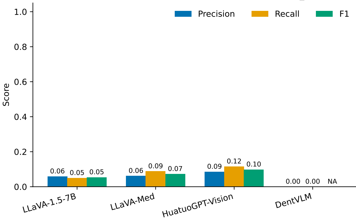
Precision, Recall, F1 (finding level) — DENTEX / few_shot
