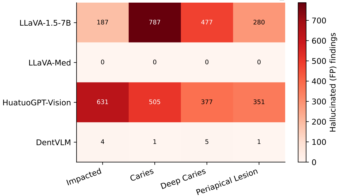
Hallucination COUNT by condition — DENTEX / zero_shot
