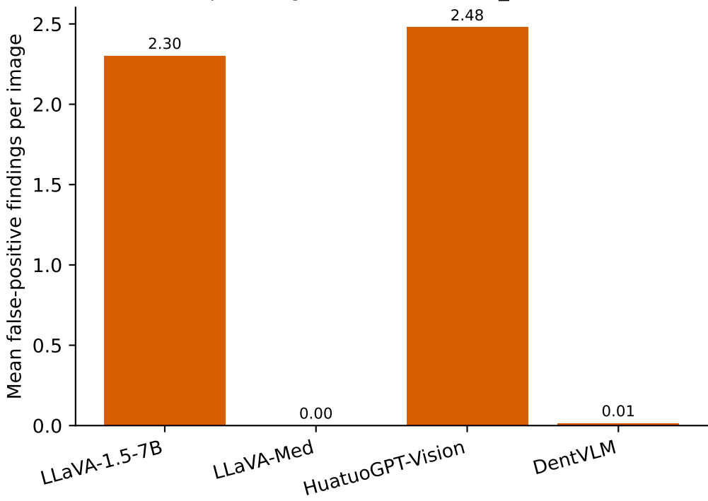
Hallucinations per image — DENTEX / zero_shot (lower is better)
