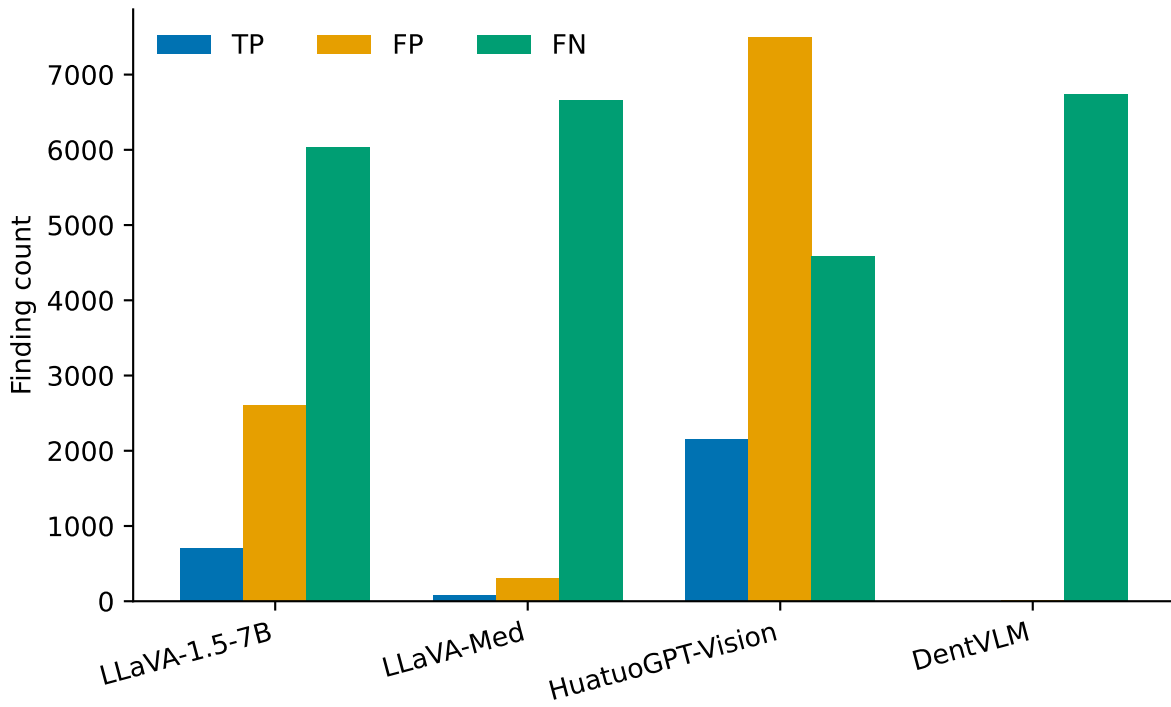
Confusion components (TP / FP / FN) — Tufts / cot TN omitted: it dwarfs these on the negative-heavy slot grid
