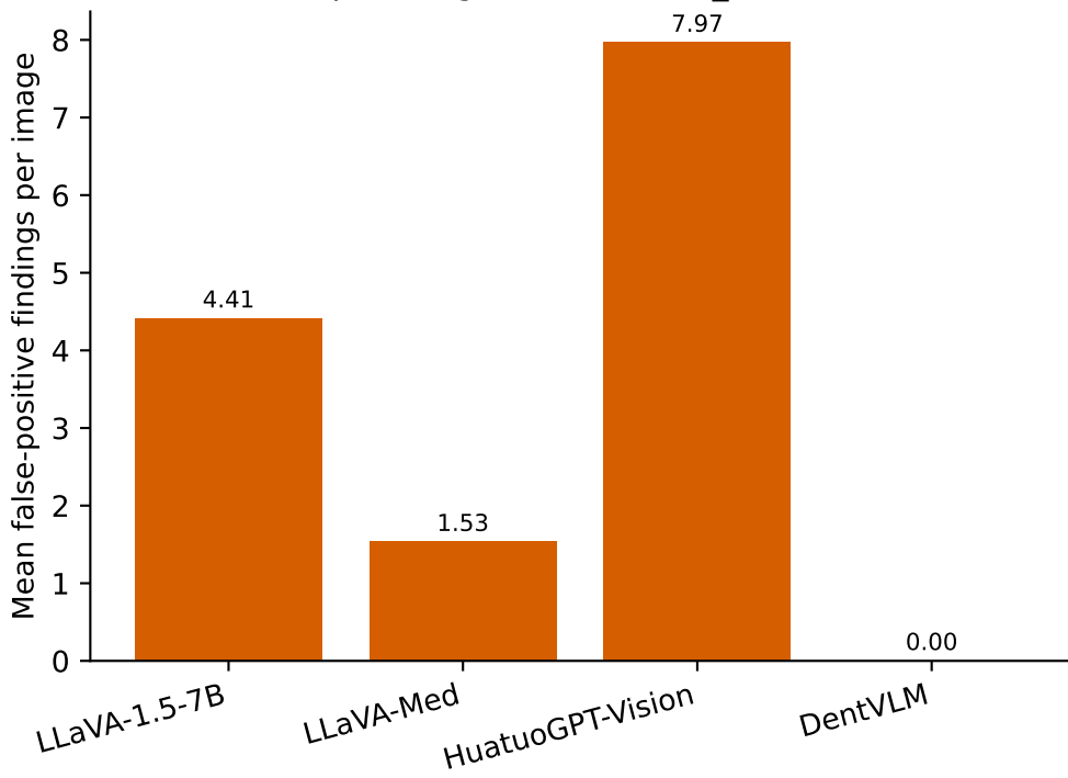
Hallucinations per image — Tufts / few_shot (lower is better)
