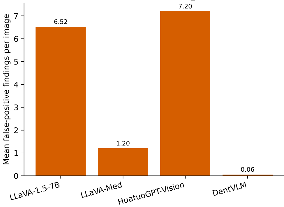
Hallucinations per image — Tufts / zero_shot (lower is better)
