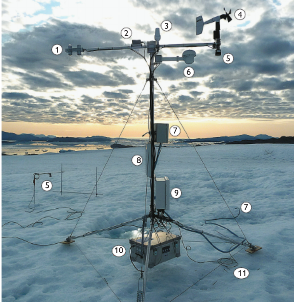
Figure 2.3: The AWS UPE_L which is part of an automated network of the Programme for Monitoring of the Greenland Ice Sheet (PROMICE). The constituents are respectively: (1) radiometer LW + SW, (2) inclinometer, (3) satellite antenna, (4) anemometer and wind vane, (5) snow depth sensor, (6) thermometer and hygrometer, (7) pressure transducer, (8) solar panel, (9) data logger and GPS, (10) battery box and (11) ground temperature sensor. Image adapted from Fausto and As 2012 .
