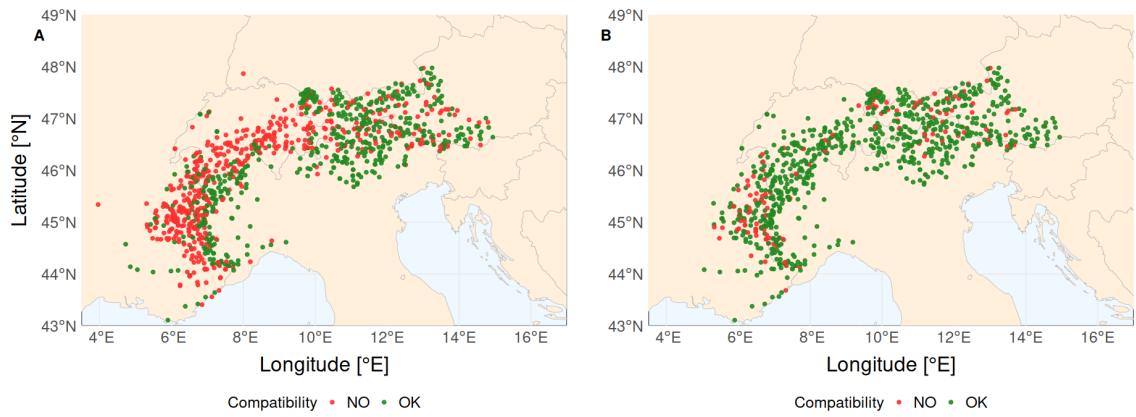
Figure 5.1: (A) Compatibility between declared station elevation and closest DEM point before checking station coordinates. (B) Compatibility between declared station elevation and closest DEM point after checking station coordinates. In both cases the ALOS AW3D30 global DEM was used: stations are labelled as compatible (OK) if the elevation difference is smaller than 12 m, namely 2/5 of pixel size.
