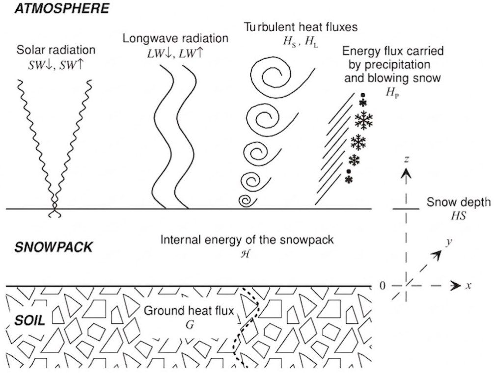
Figure 2.3: Schematic representation of the energy balance of a snowpack. Shortwave (SW) and longwave (LW) radiation, originating from the Sun and from thermal emission respectively, make up the net radiative budget R_N . The internal energy of the snowpack \mathcal{H} can also be altered by the turbulent heat fluxes H_S and H_L , the precipitation heat flux H_P and the ground heat flux G . Image adapted from Armstrong and Brun 2008.
