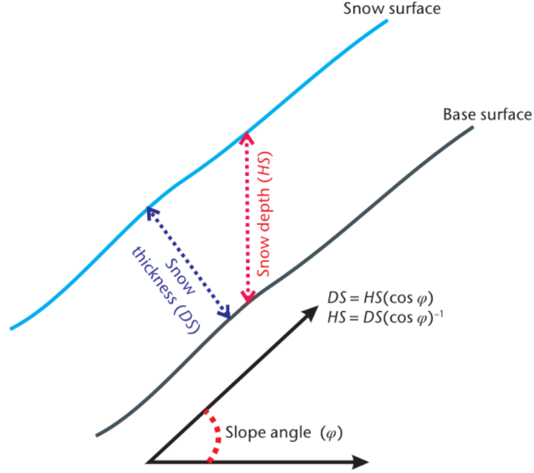
Figure 2.4: Relationship between snow depth (HS) and snow thickness (DS) on a slope. Image adapted from WMO 2024.
