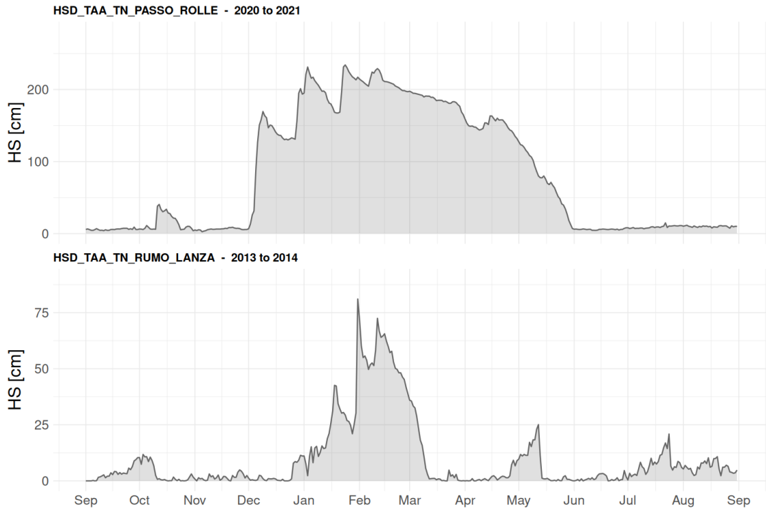
Figure 5.5: (a) HS series which exhibits a ground level misidentification, with summer values constant at \sim 10 cm. (b) HS series which exhibits summer spikes and misreading, given that Rumo Lanza stands at 1100 m a.s.l. and clearly can't experience snow cover during the hottest months.
