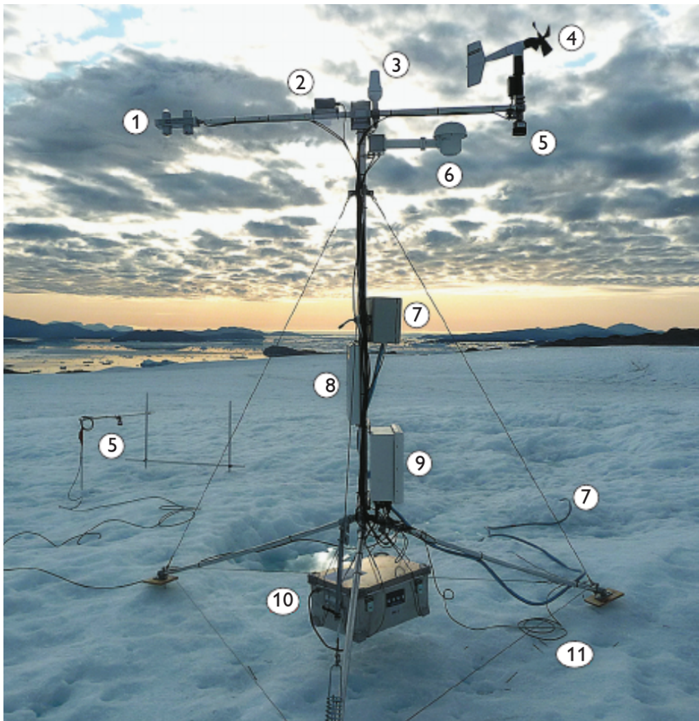
Figure 2.5: The AWS UPE_L which is part of an automated network of the Programme for Monitoring of the Greenland Ice Sheet (PROMICE). The constituents are respectively: (1) radiometer LW + SW, (2) inclinometer, (3) satellite antenna, (4) anemometer and wind vane, (5) snow depth sensor, (6) thermometer and hygrometer, (7) pressure transducer, (8) solar panel, (9) data logger and GPS, (10) battery box and (11) ground temperature sensor. Image adapted from Fausto and As 2012 .
