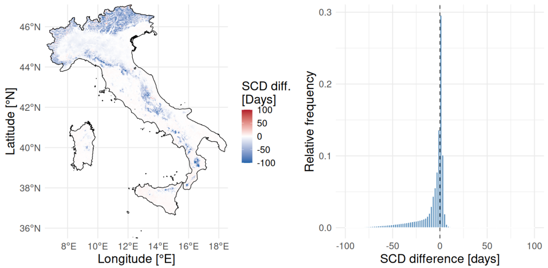
Figure 3.10: MODIS
