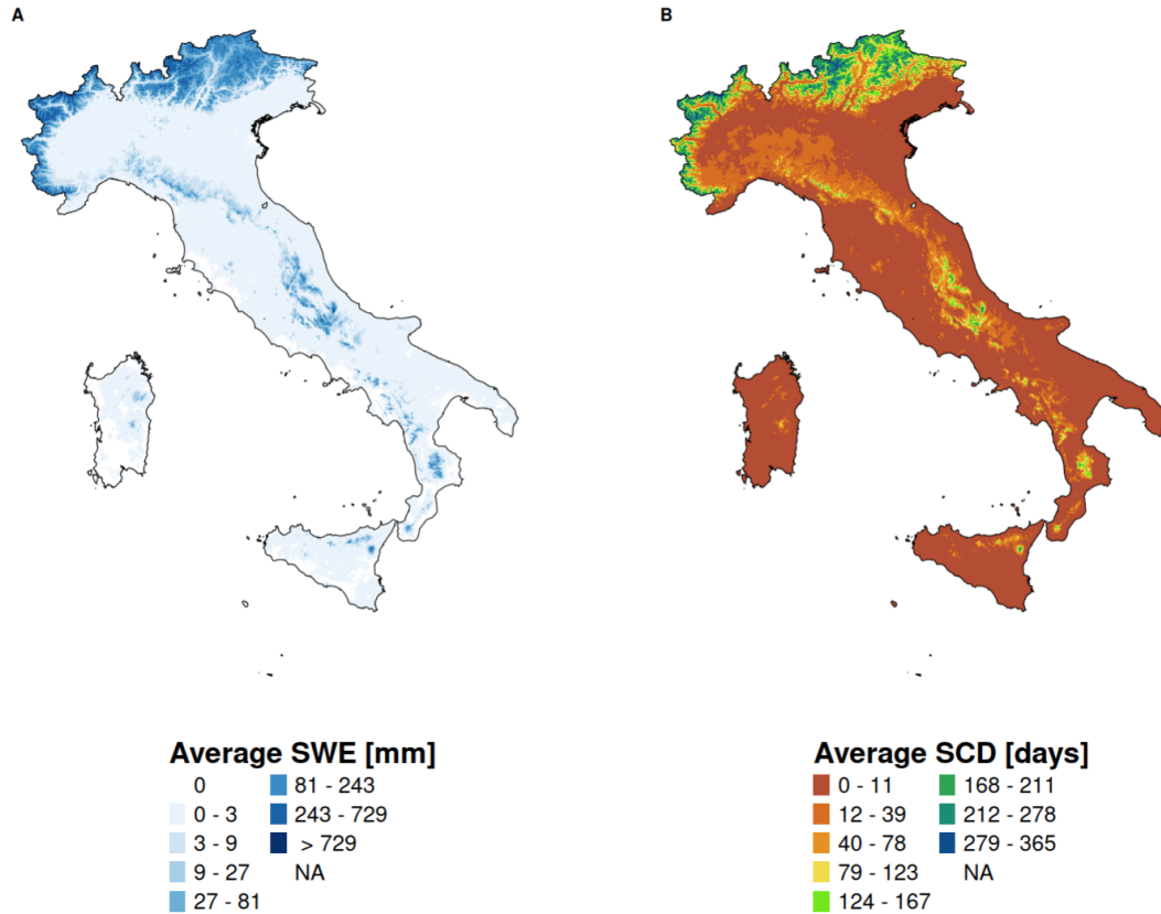
Figure 3.8: (a) Average seasonal snow water equivalent (SWE), computed as the mean of the November–June averages of each hydrological year over the period 1 September 2010–31 August 2025. (b) Average snow cover duration (SCD), computed as the mean of the annual SCD maps across the same period.
