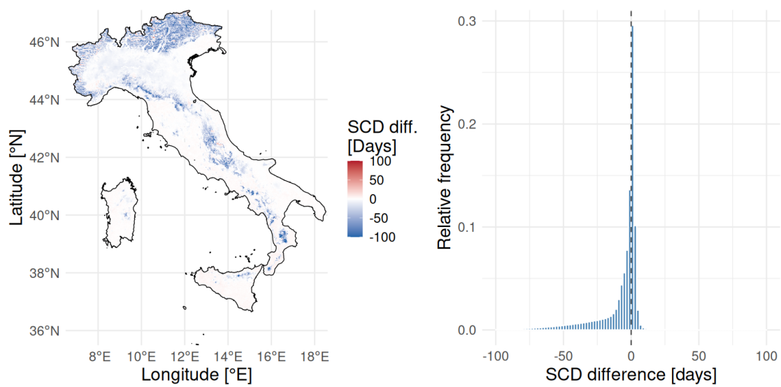
Figure 3.9: MODIS
