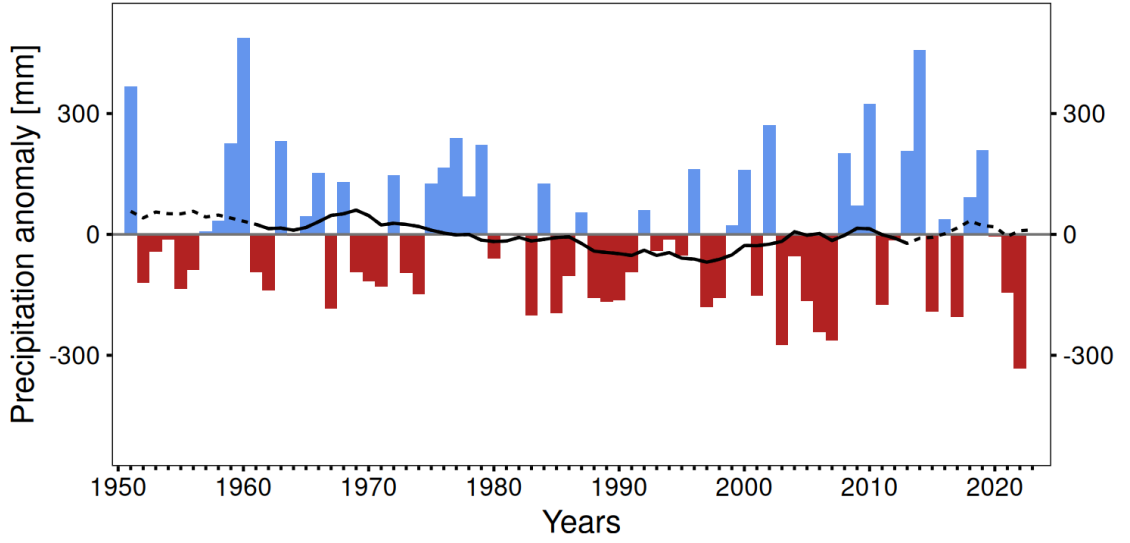
Figure 4.3: Annual precipitation anomalies [mm] averaged over the Italian Hydrological part of the Greater Alpine Arc (IH-GAR) for the period 1951–2023, relative to the 1991–2020 climatology. Blue (red) bars indicate positive (negative) anomalies. The black line is a 21-year running mean: its dashed segments, at the beginning and at the end of the record, are computed over a truncated time window.
