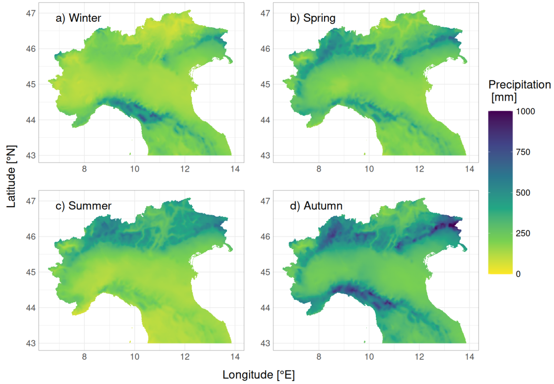
Figure 4.2: Seasonal precipitation climatology for the Italian Hydrological part of the Greater Alpine Arc (IH-GAR), computed over the 1991–2020 period at a spatial resolution of 30 arc-seconds. Autumn is the wettest season on average over the lowlands and the Alpine foothills, whereas the internal Alps experience enhanced precipitations during summer.
