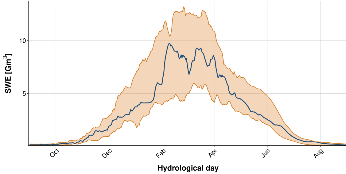
Figure 3.3: Total SWE climatologies.
