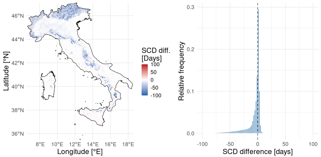
Figure 3.9: MODIS
