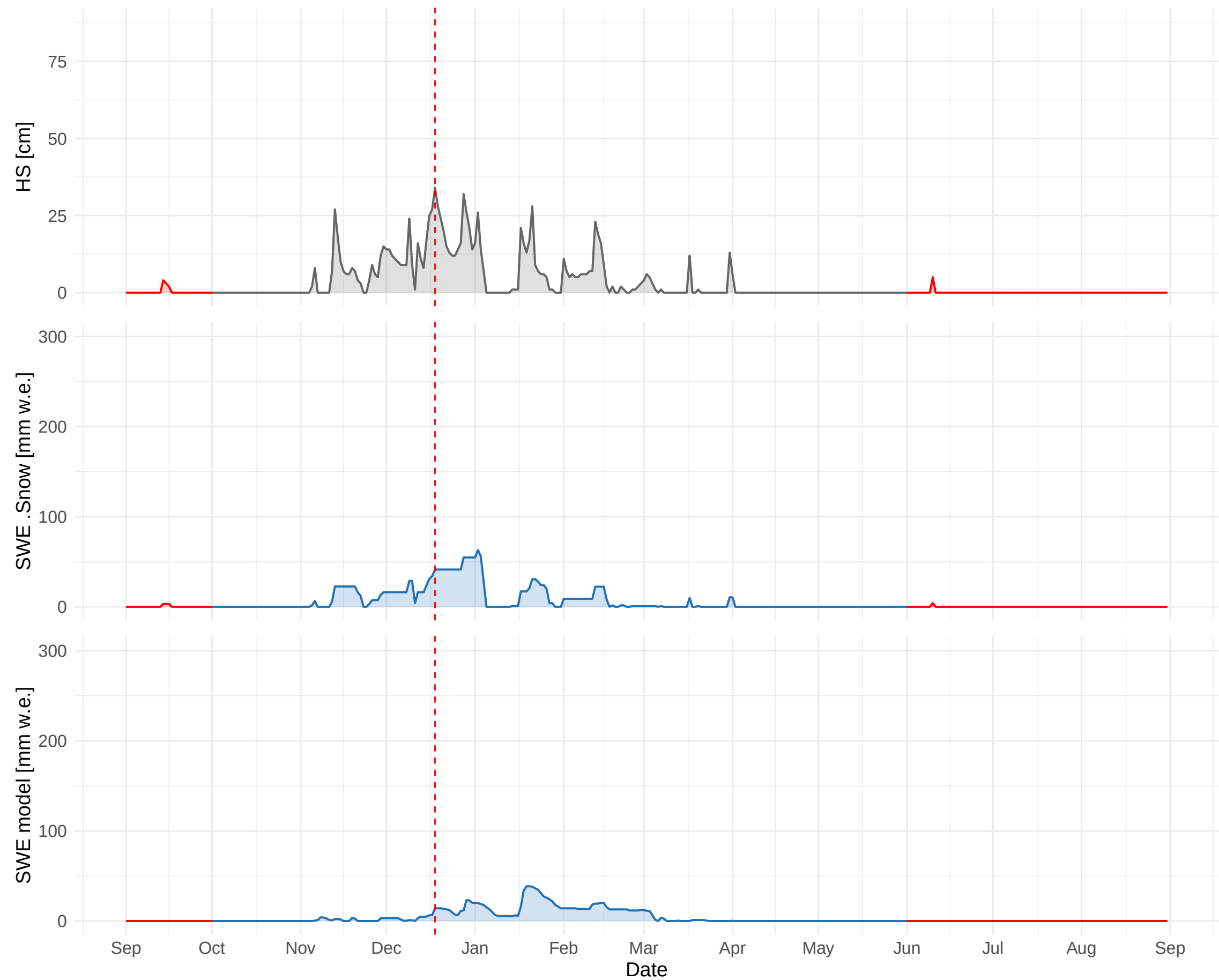
HSD_CH_ABO (1321 m a.s.l.) – 2017 to 2018
