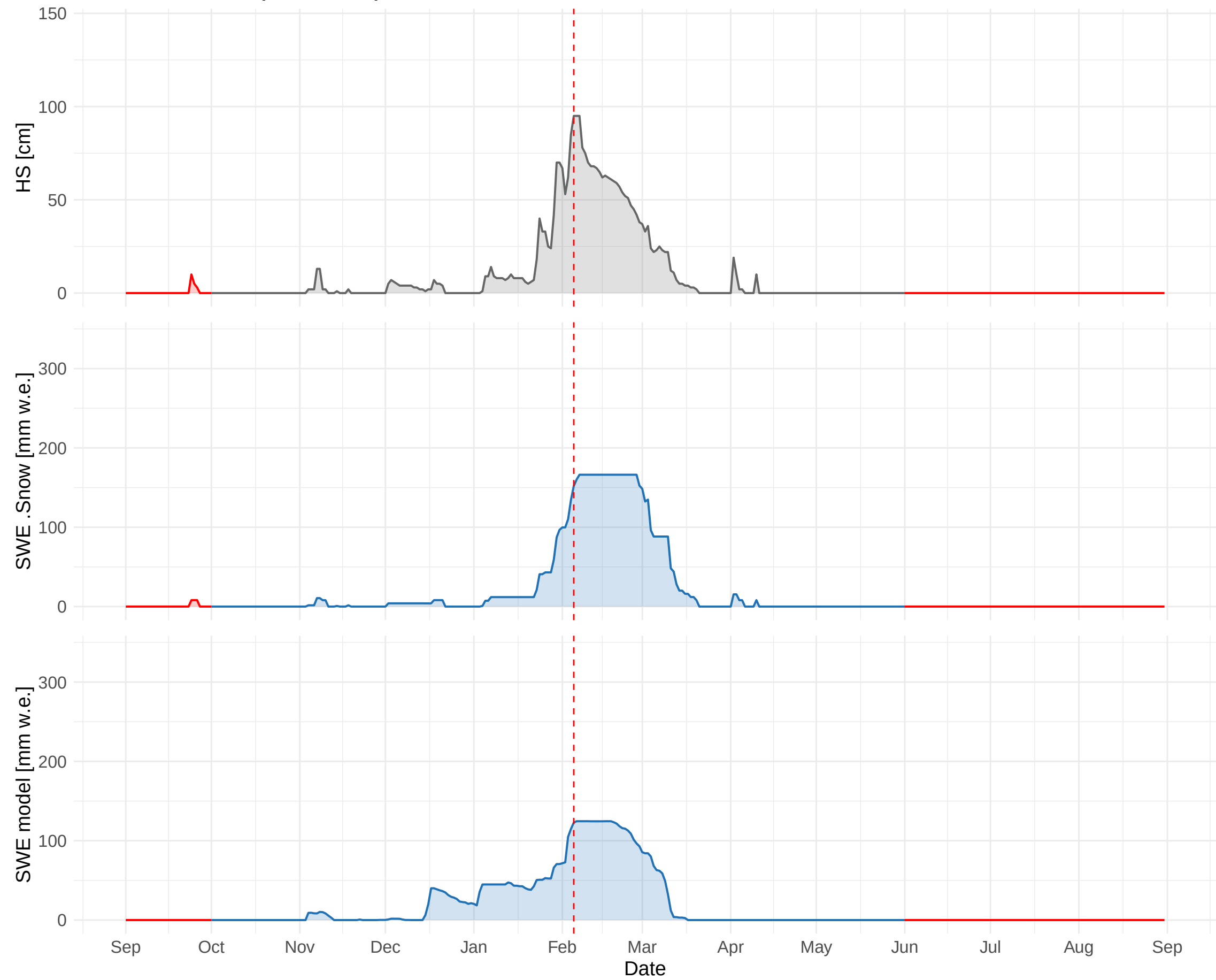
HSD_CH_ABO_MAN (1321 m a.s.l.) – 2002 to 2003
