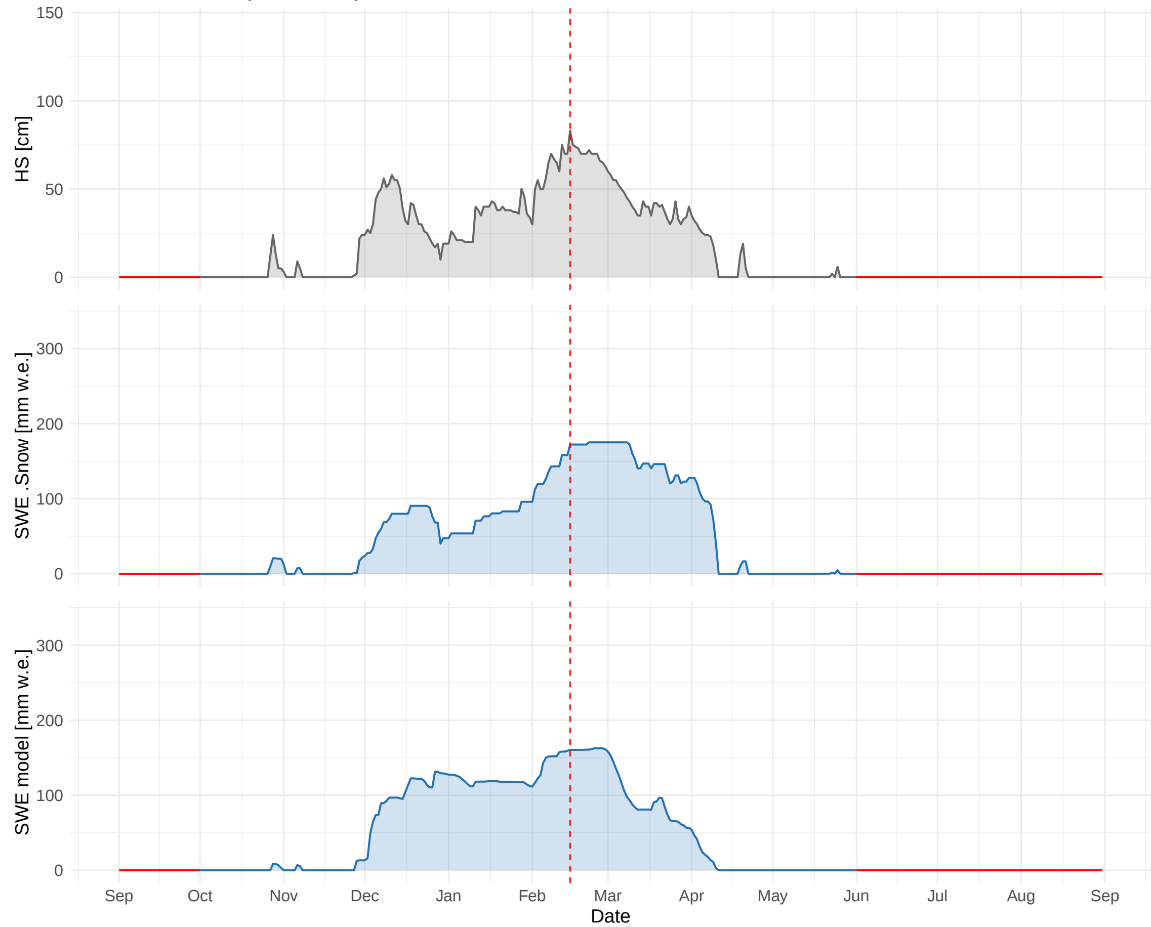
HSD_CH_ABO_MAN (1321 m a.s.l.) – 2012 to 2013
