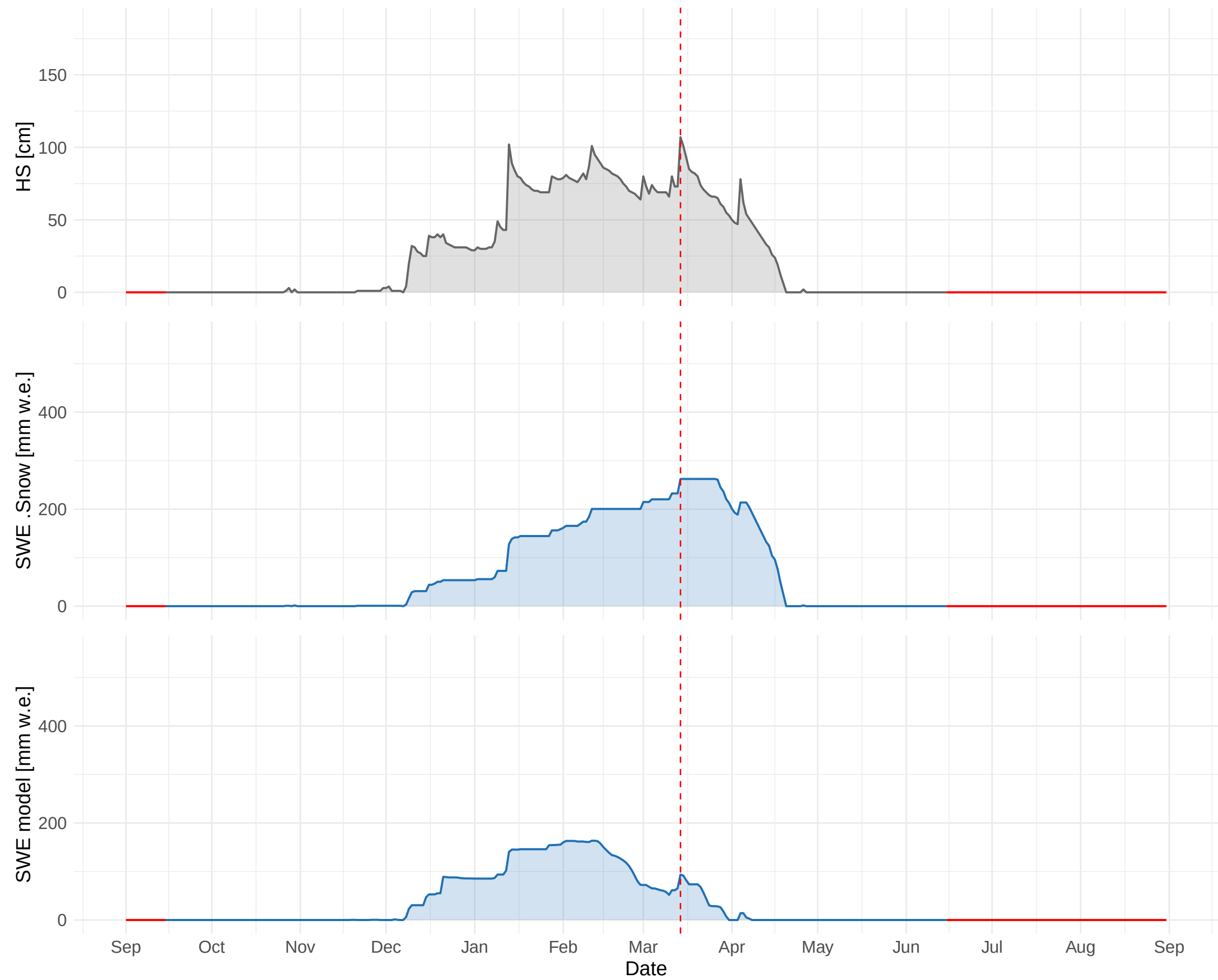
HSD_CH_BLA (1538 m a.s.l.) – 2018 to 2019
